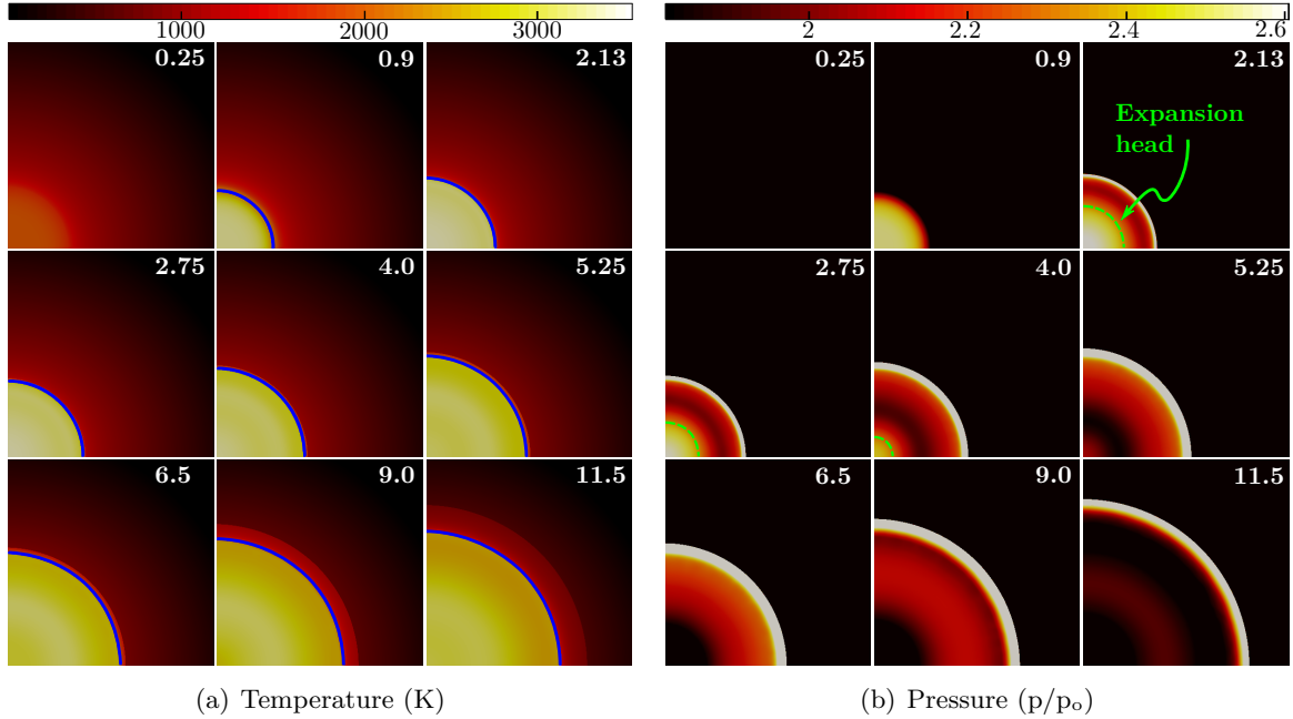
Figure 5.12 Select time steps of temperature contours for the (a) Temperature (K) and (b) Pressure ( p/p_o ) for the circular case with \tau_e/t_a = 0.1 . Time in upper-right corner of each frame is normalized time, (t - \tau_i)/\tau_e .
