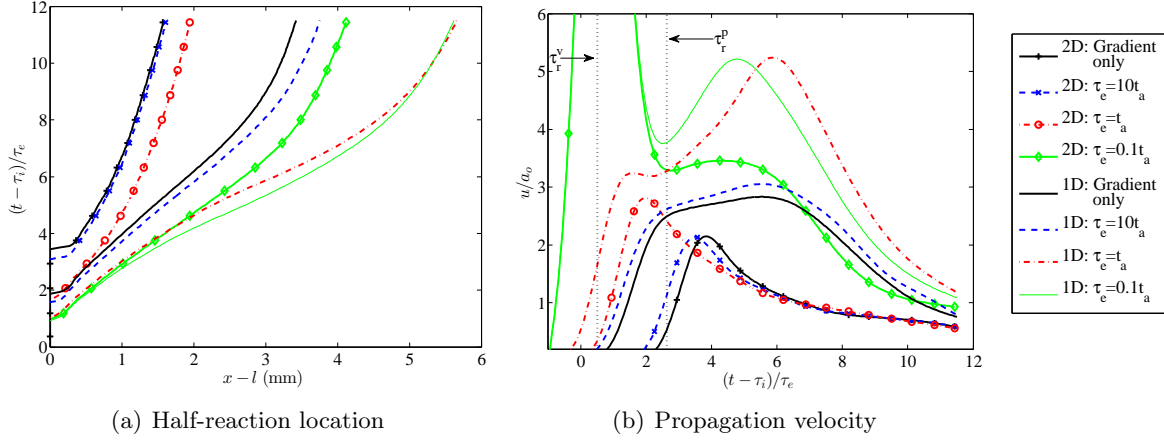
Figure 5.13 Circular model: comparison of half-reaction location, propagation velocity of reaction wave, and global heat release along the x -axis of all 2-D cases. Corresponding 1-D cases are included with the same line style and color sans markers. Two vertical dotted lines are included to represent the reaction times for an isochoric, \tau_r^v , and isobaric, \tau_r^p , homogeneous reactor.
