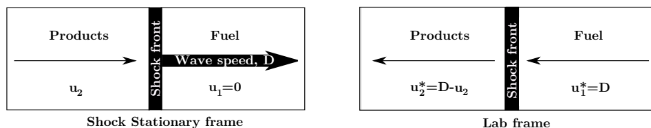
Figure 3.1 Sketch of the flow properties ahead and behind a detonation wave in the shock stationary reference frame (left) and lab reference frame (right).
