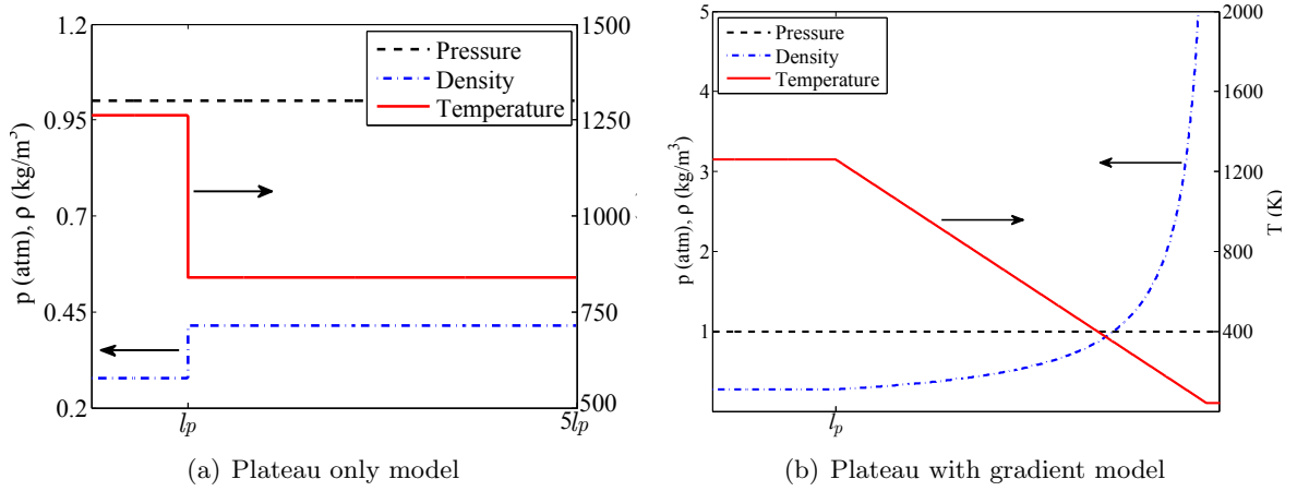
Figure 3.2 Initial conditions for hot spot models.
