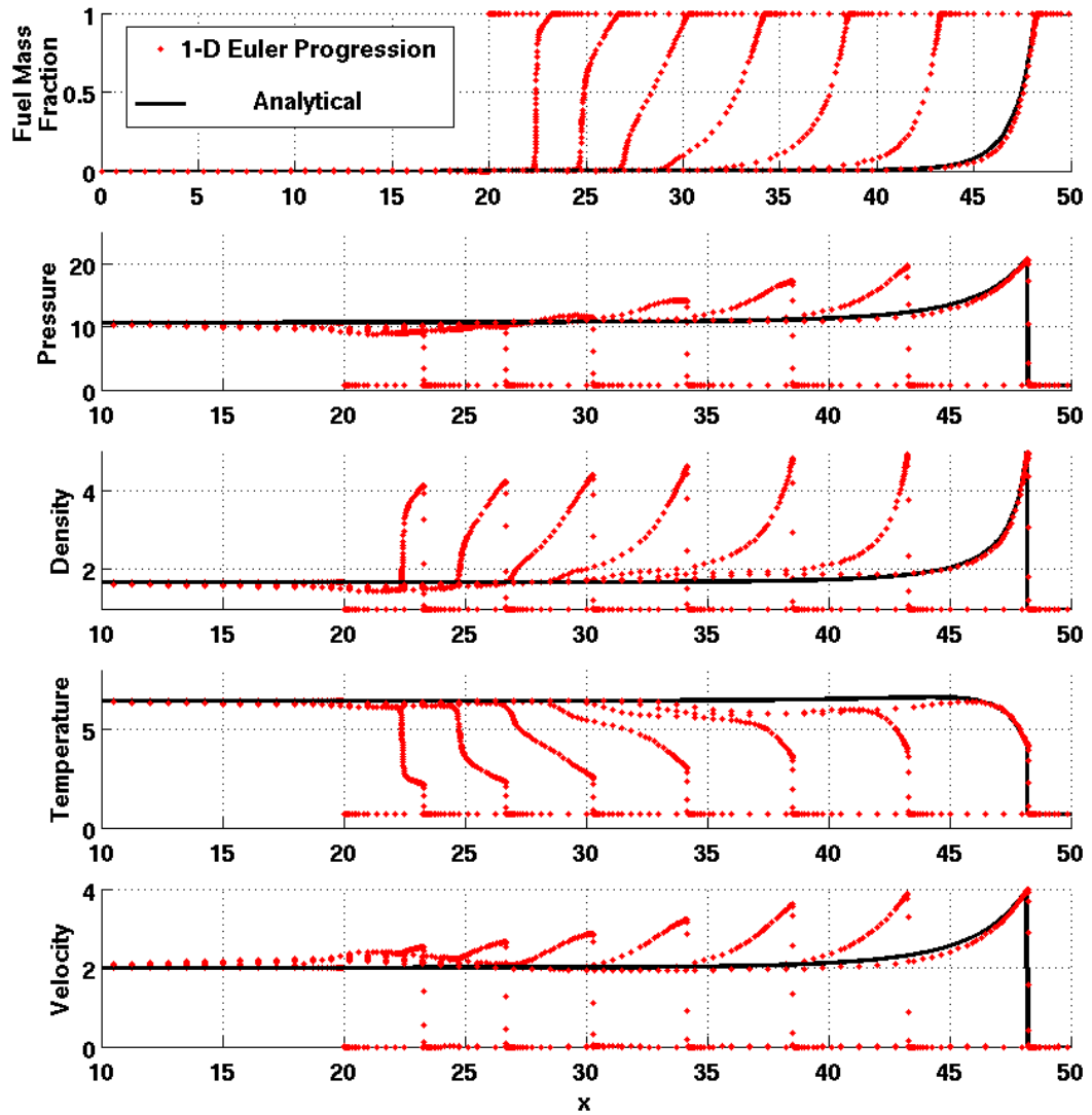
Figure 4.2 Progression of the 1-D Euler solution from t = 0 to t = 7
