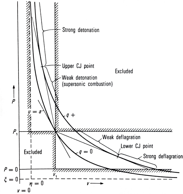
Figure 1.1 Rankine-Hugoniot curve[2]
